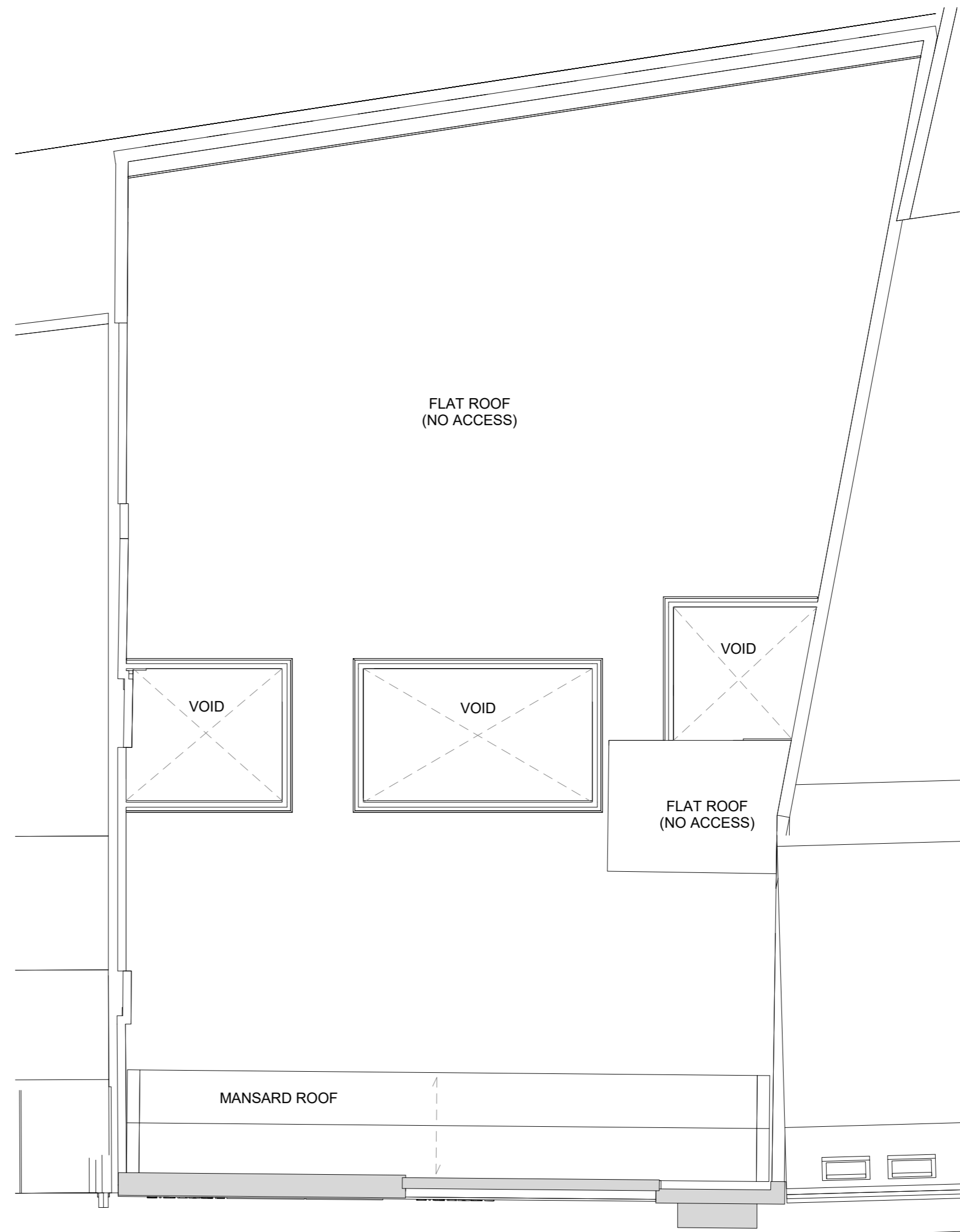
2 04001 ROOF LEVEL - GA PLAN 00102 1 1 : 100
